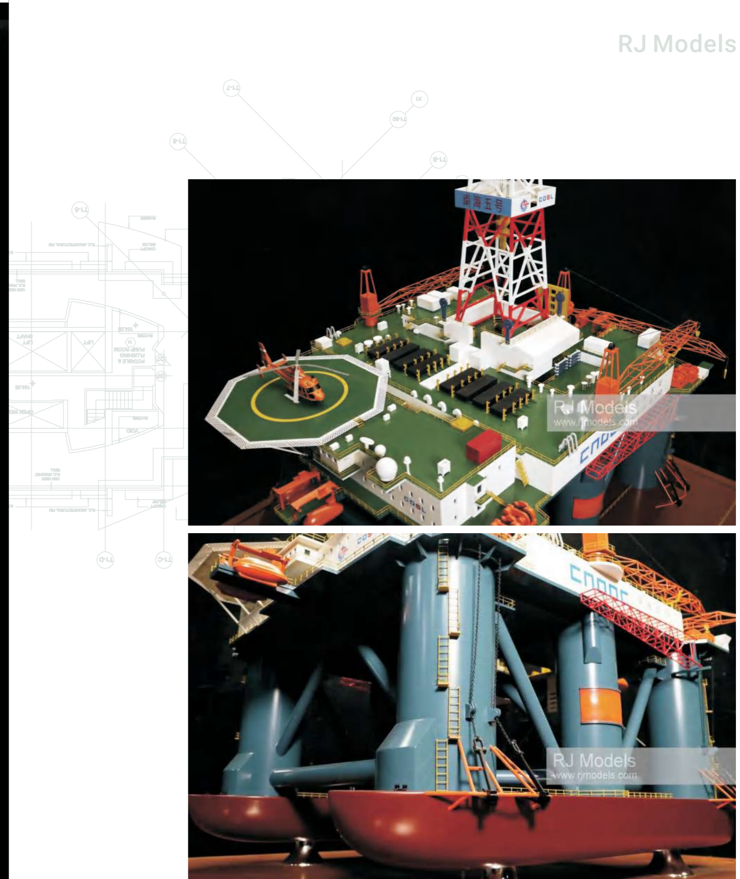
Oil Drilling, South China Sea COSL 1:100
