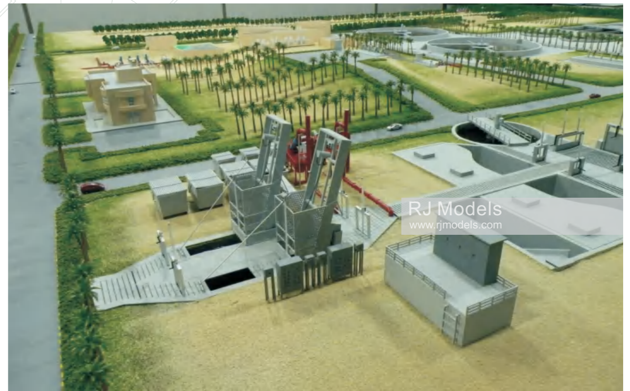
Sewage Treatment, Jordan 1:75
